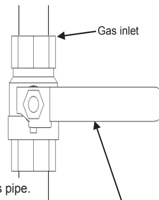
Manual Gas Valve Shown in the "OFF" Position
