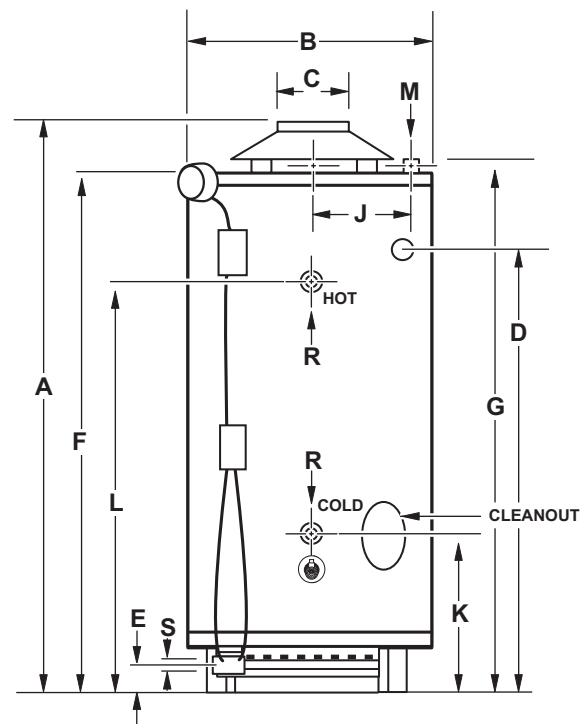
Water Connections Top and Front
