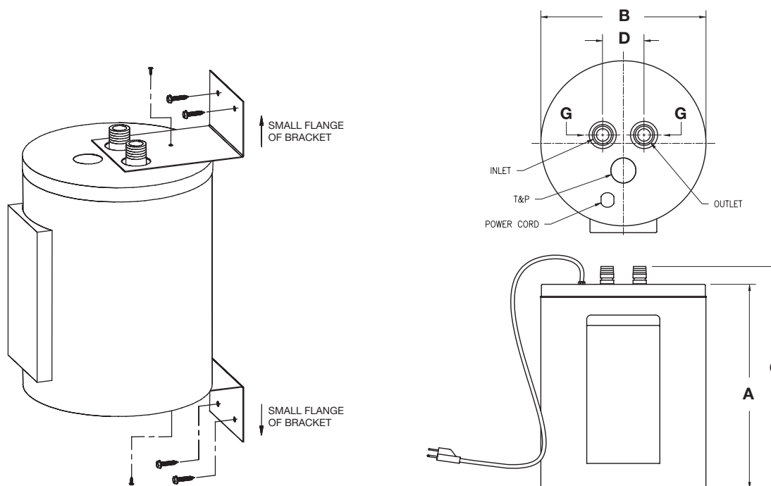
Optional Wall Mounting Bracket (2 brackets) Part Number 265-45018-00
