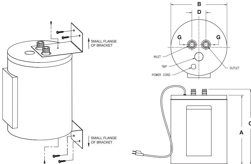
Optional Wall Mounting Bracket (2 brackets) Part Number 265-45018-00
