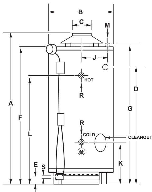
Water Connections Top and Front
