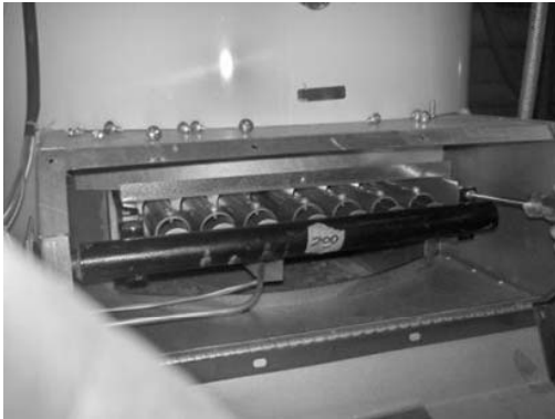
Step 7: Remove manifold bracket screws
