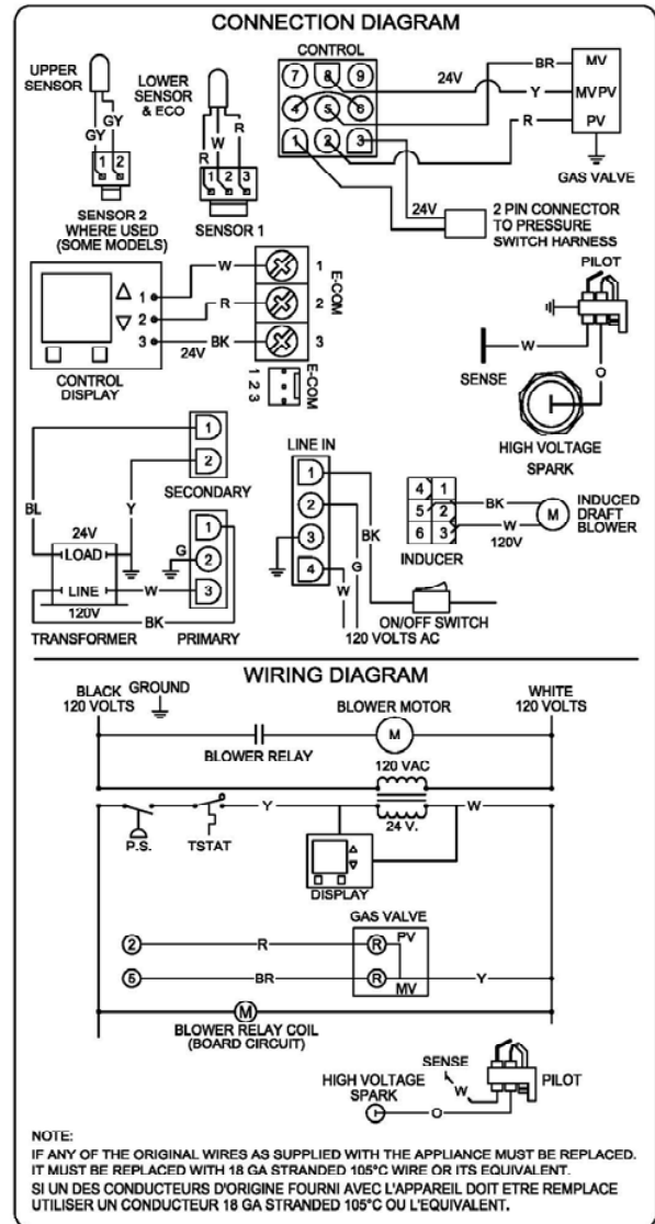
WIRING DIAGRAM
