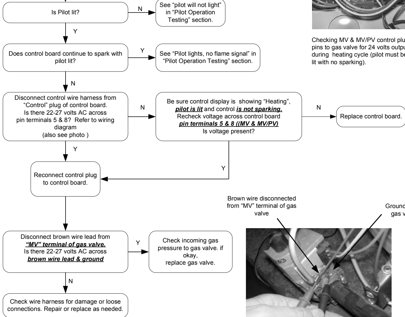
Checking main valve (MV) voltage to gas valve.
