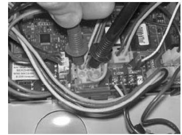
Checking MV & MV/PV control plug pins to gas valve for 24 volts output during heating cycle (pilot must be lit with no sparking).
