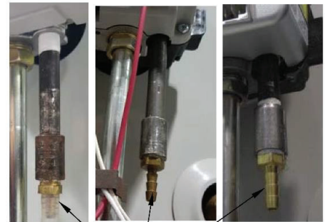
PRESSURE TAP SHOWN INSTALLED
