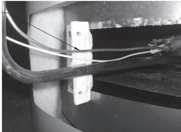
Thermocouple position
