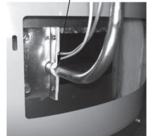
POSITION THERMOCOUPLE/THERMOPILE, PILOT TUBE AND PIEZO WIRE
