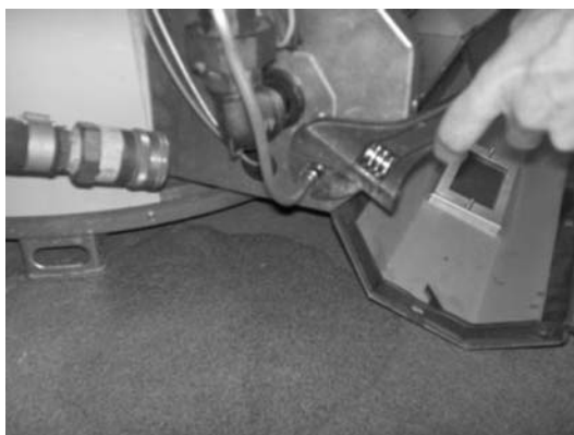
Step 3: Disconnect Pilot Fitting from Burner Box
