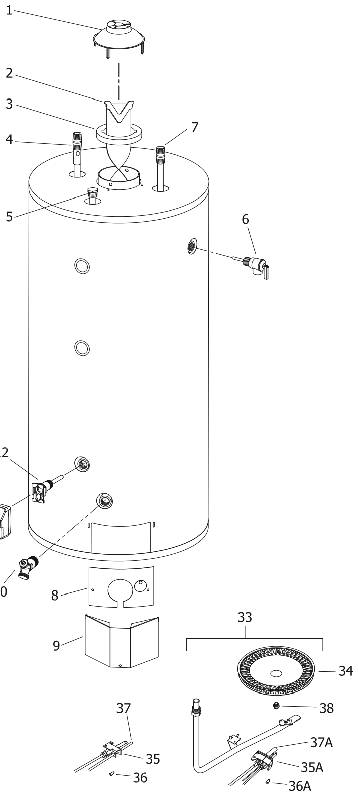
LP GAS (SX) BURNER ASSEMBLY
