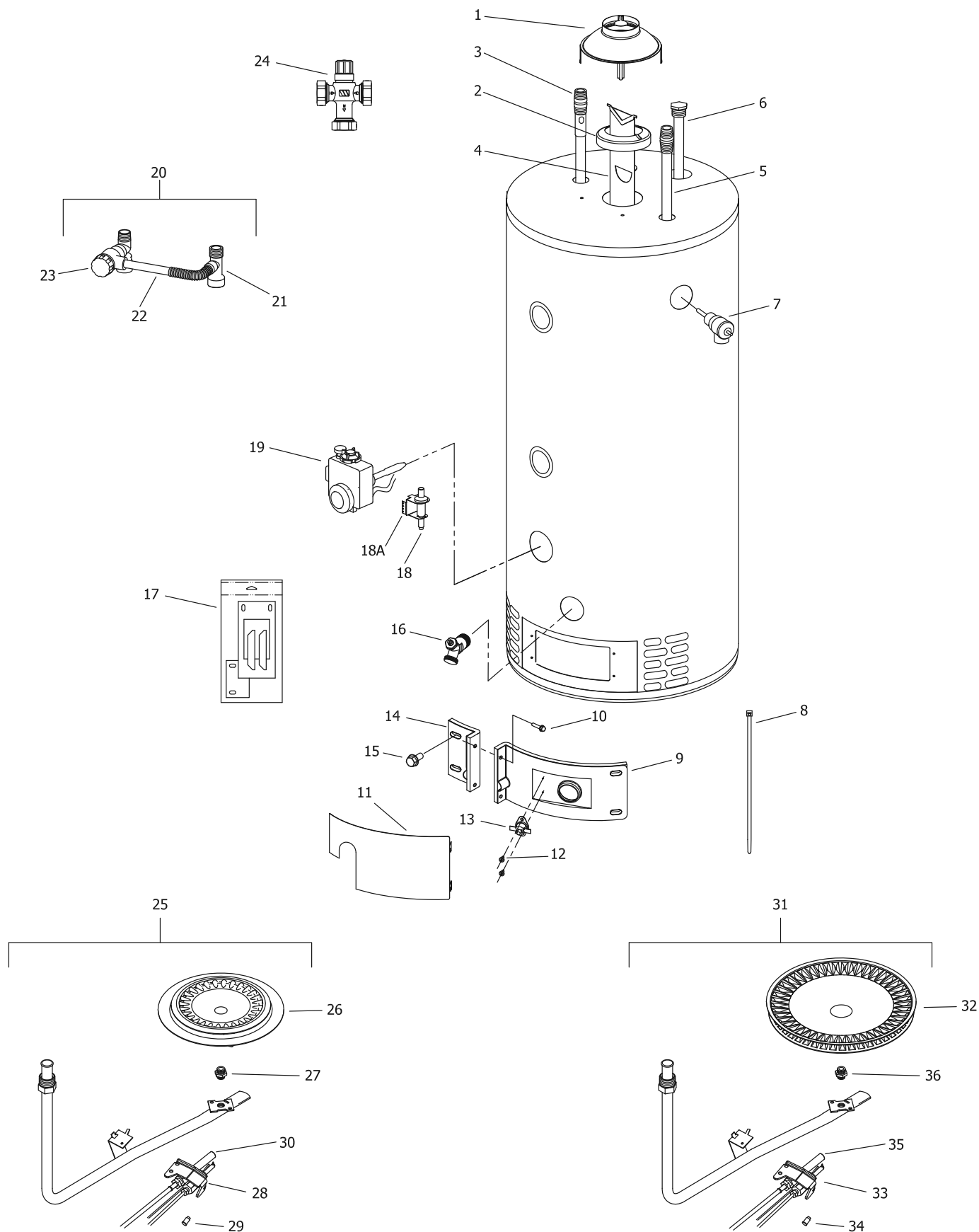
NATURAL GAS (BN) BURNER ASSEMBLY
