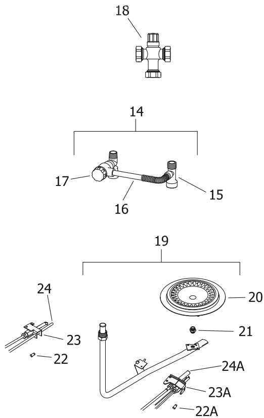
NATURAL GAS (BN) BURNER ASSEMBLY
