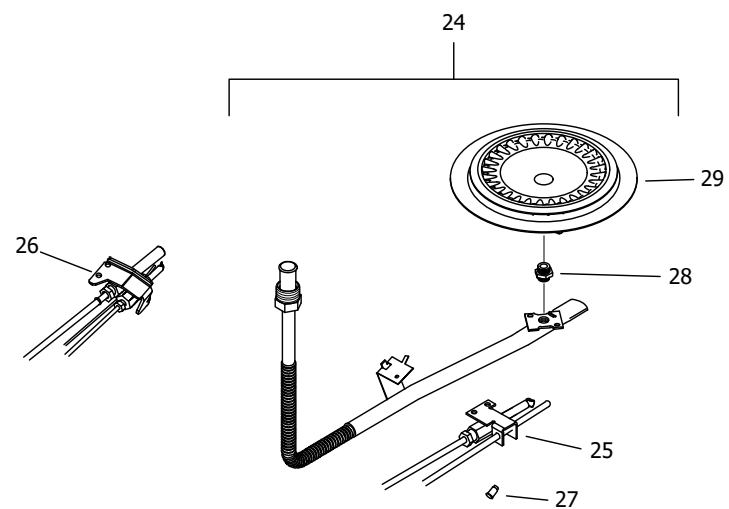
NATURAL GAS (BN,CN) BURNER ASSEMBLY
