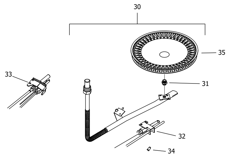
LP GAS (SX,CX) BURNER ASSEMBLY
