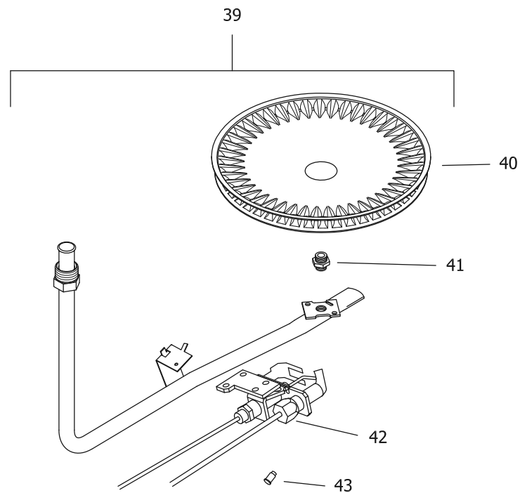
LP GAS (SX) BURNER ASSEMBLY
