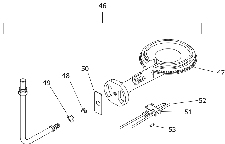
LP GAS (CX) BURNER ASSEMBLY
