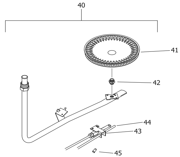
LP GAS (SX) BURNER ASSEMBLY
