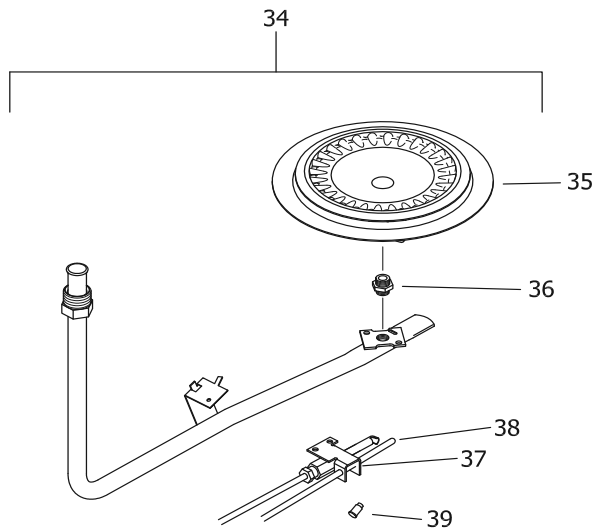
NATURAL GAS (BN) BURNER ASSEMBLY
