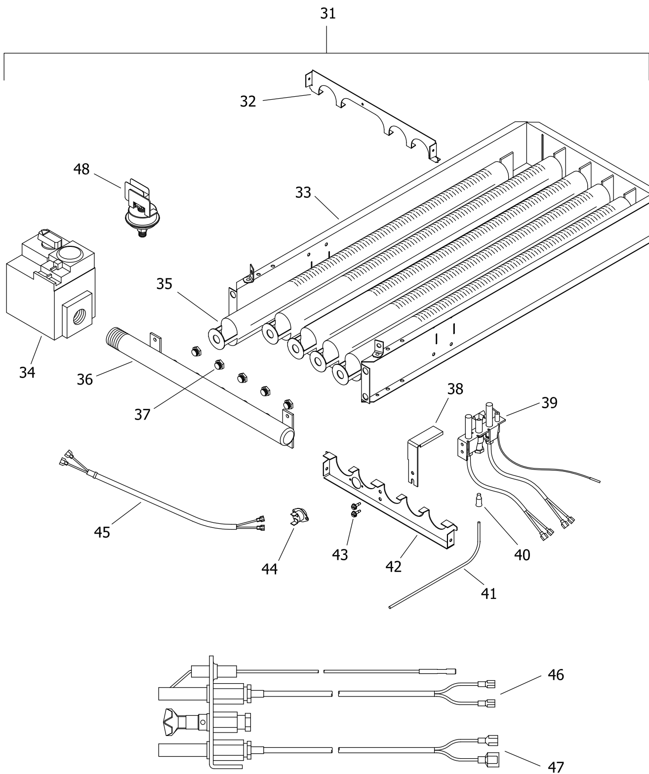
THERMOPILE DETAIL
