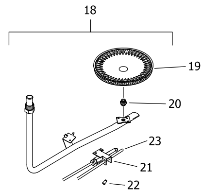
LP GAS (SX) BURNER ASSEMBLY
