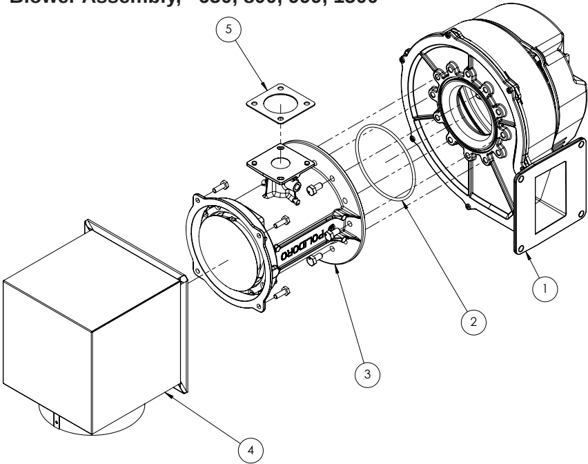
Blower Assembly, 650, 800, 999, 1500
