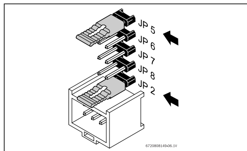
Fig. 7 Jumper configuration
