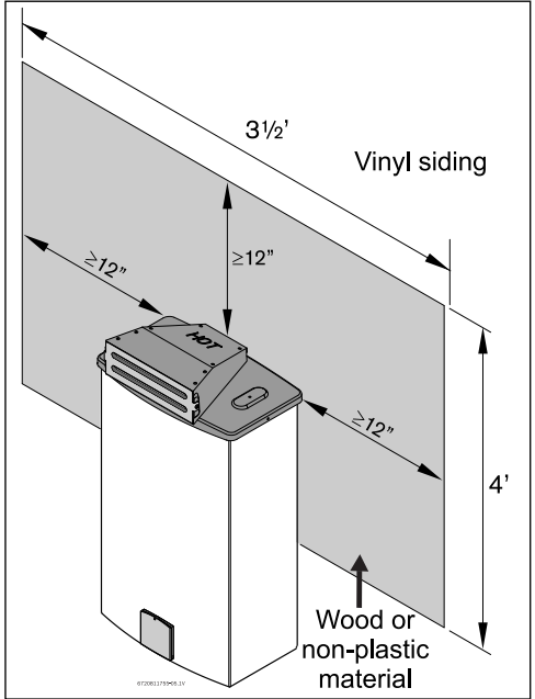
Fig. 10 Installation on vinyl siding
