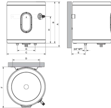
Dimensions for Wall Hung Models
