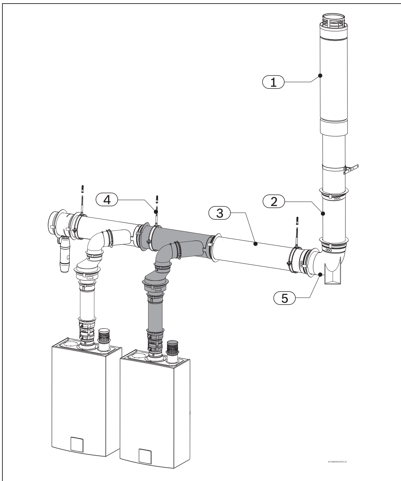
Fig. 12 Vertical setup - for horizontal termination see Fig. 21
