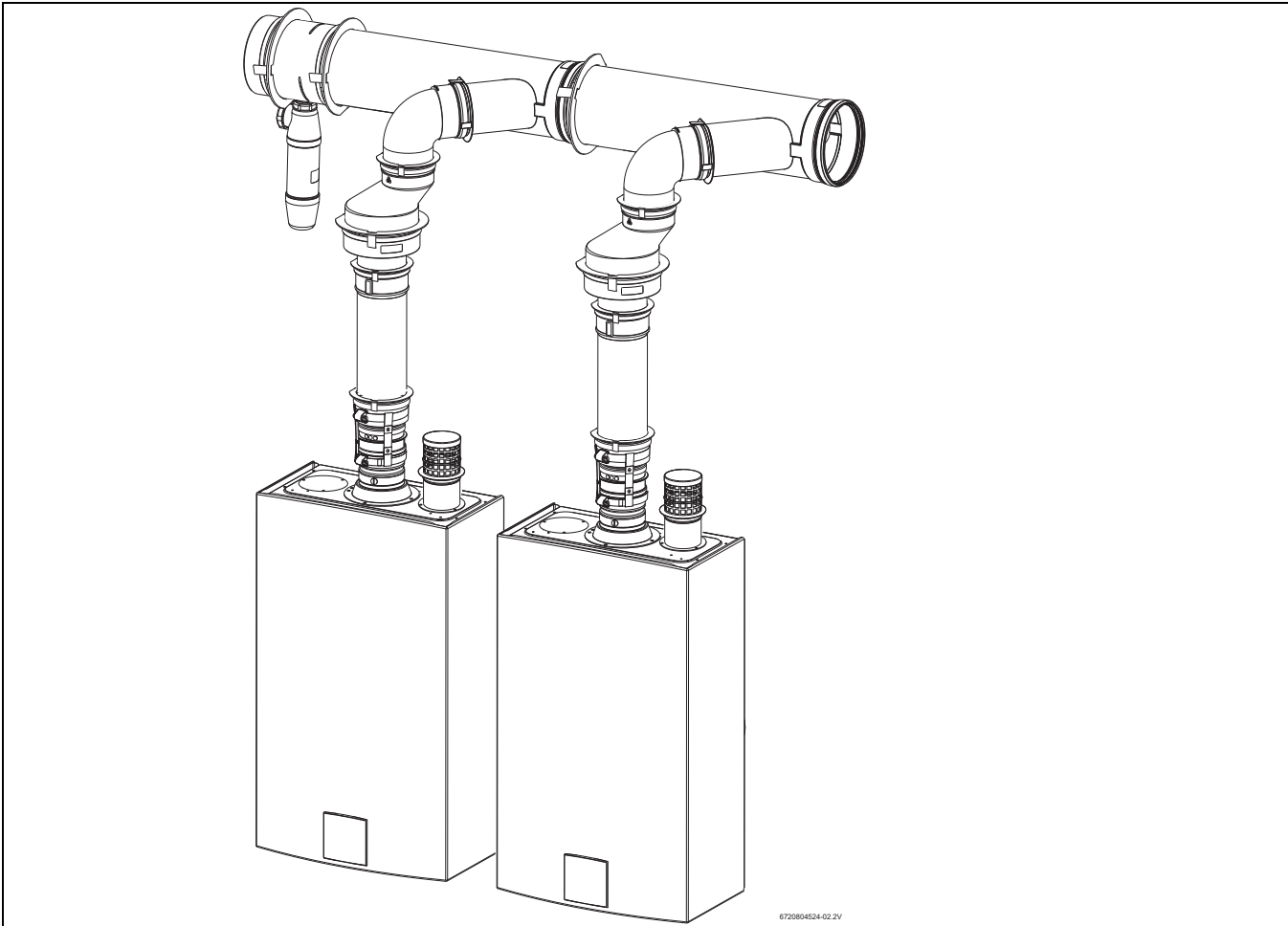
Fig. 11 Complete remainder of vent pipe installation identically to the first heater. Repeat for up to 4 units total.
