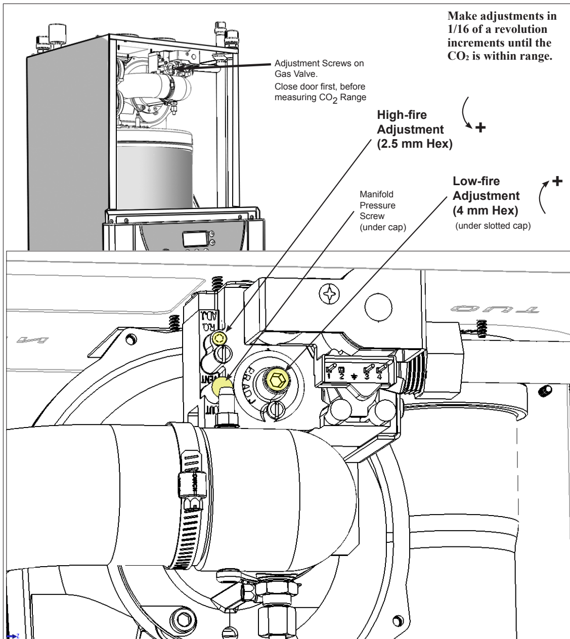
Figure 25. Adjustment Screws and Settings for CO 2 (Wall Mounted Brute LX)
