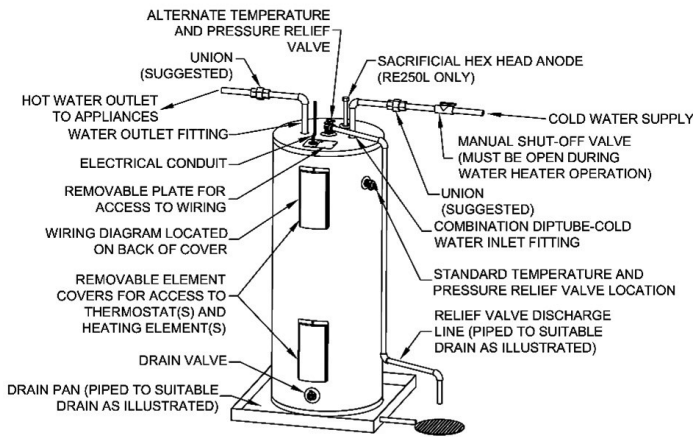
Fig. 3 Top Inlet Models
