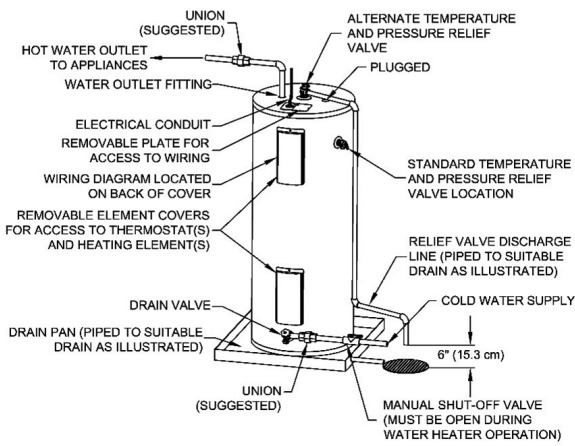
Fig. 4 Bottom Inlet Models
