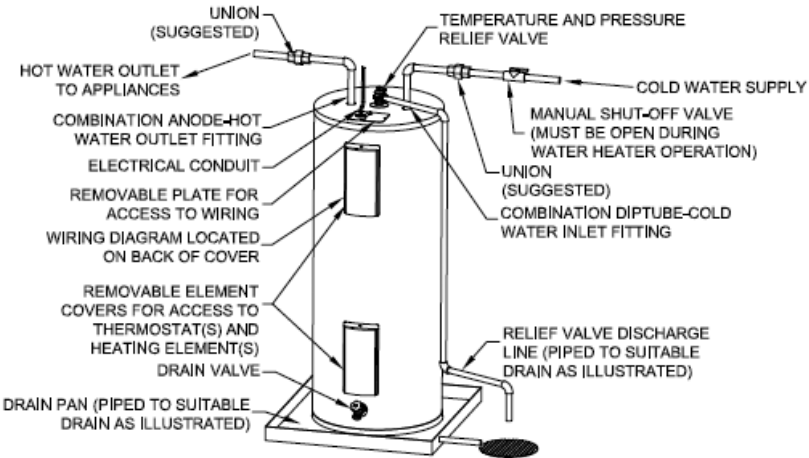
Fig. 1 Top Inlet Models
