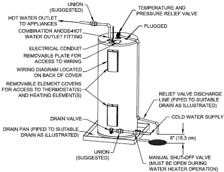
Fig. 2 Bottom Inlet Models
