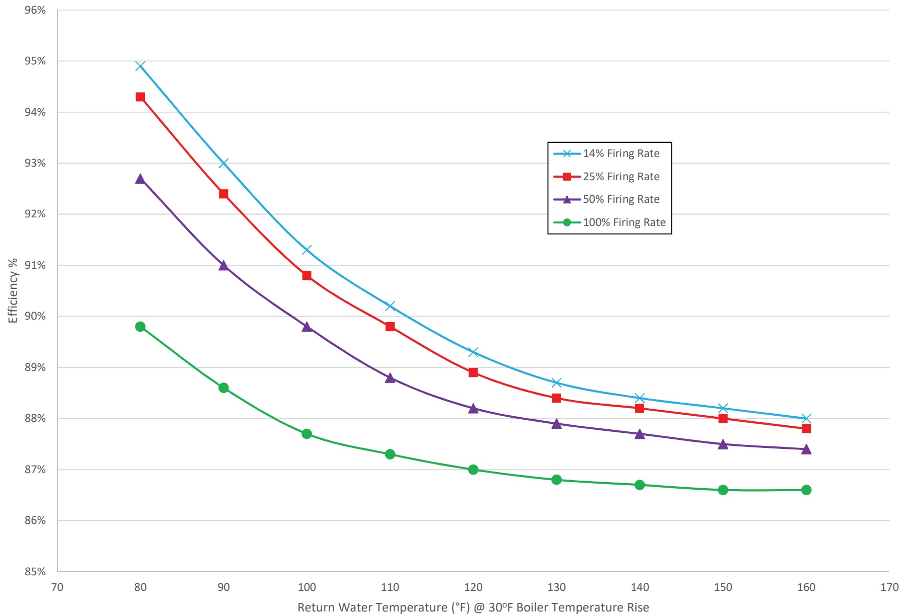
OmniTech Model BOC Efficiency Curve
